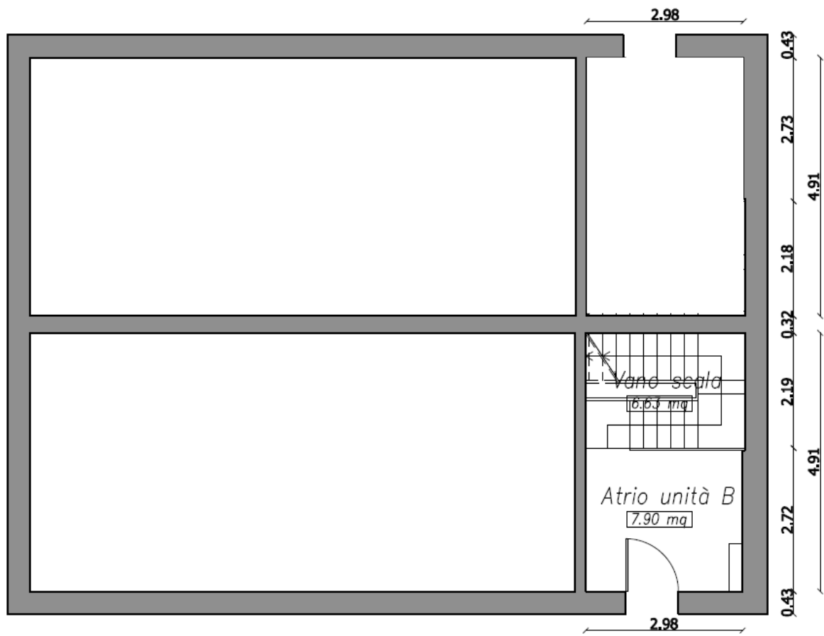
Piano terra
