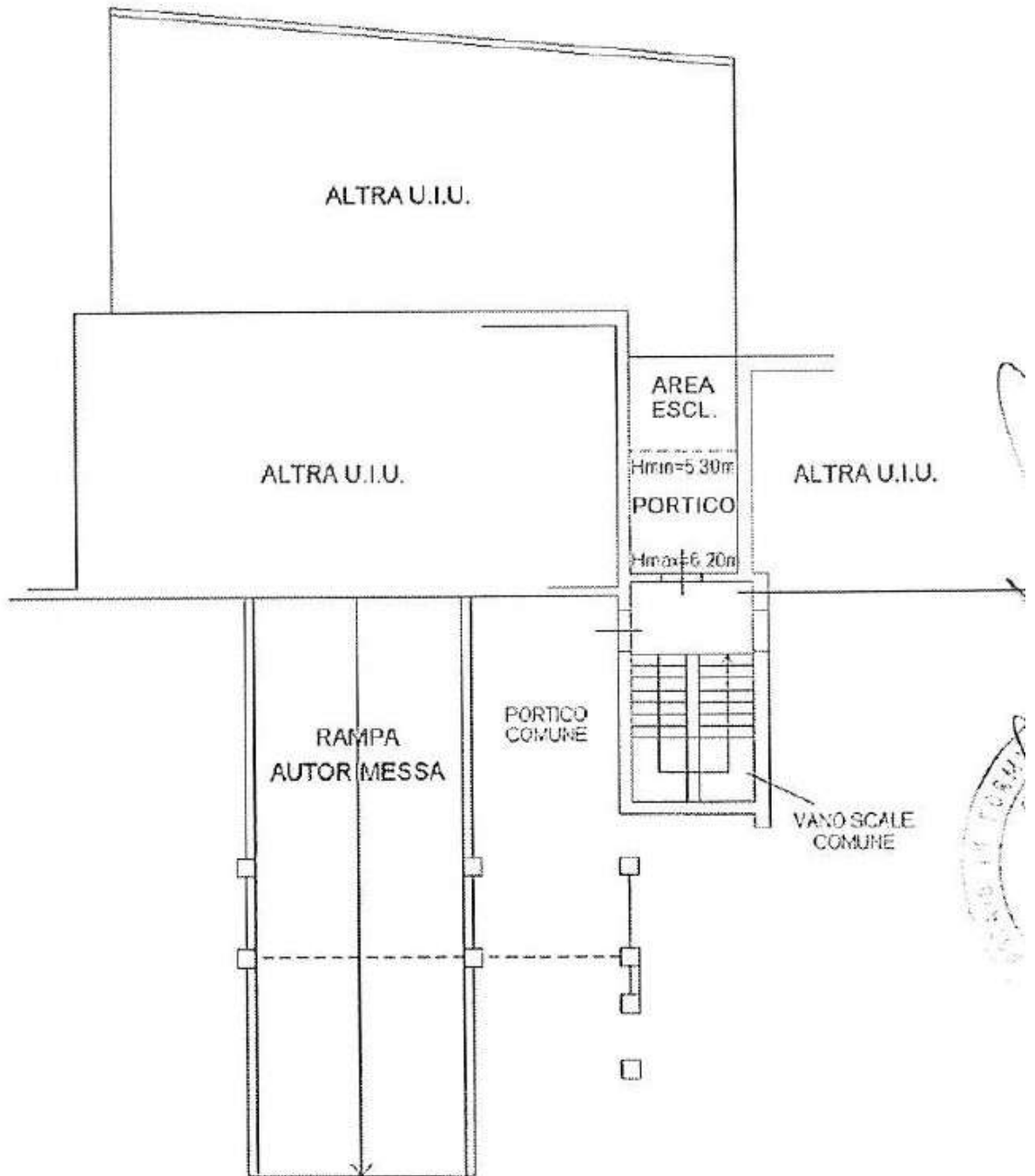
PIANO TERRA
