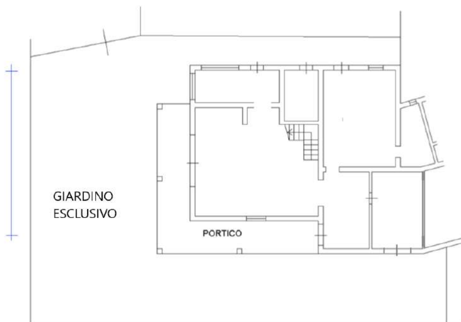
PIANO TERRA H=2.70
