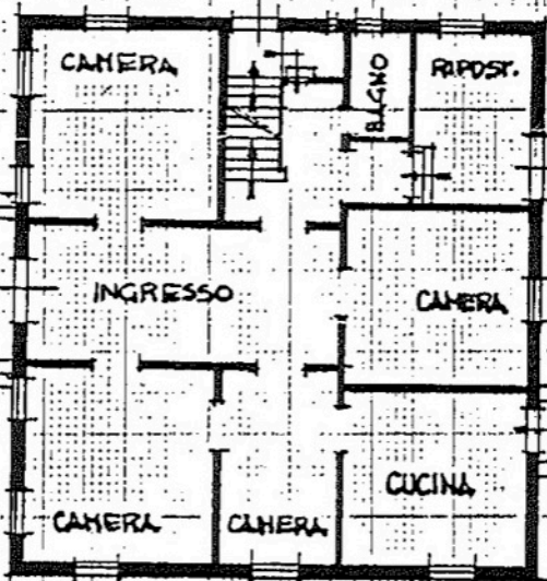
PIANO TERRA H= ml. 3,50
