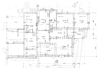
PIANO TERRA - 1:100
